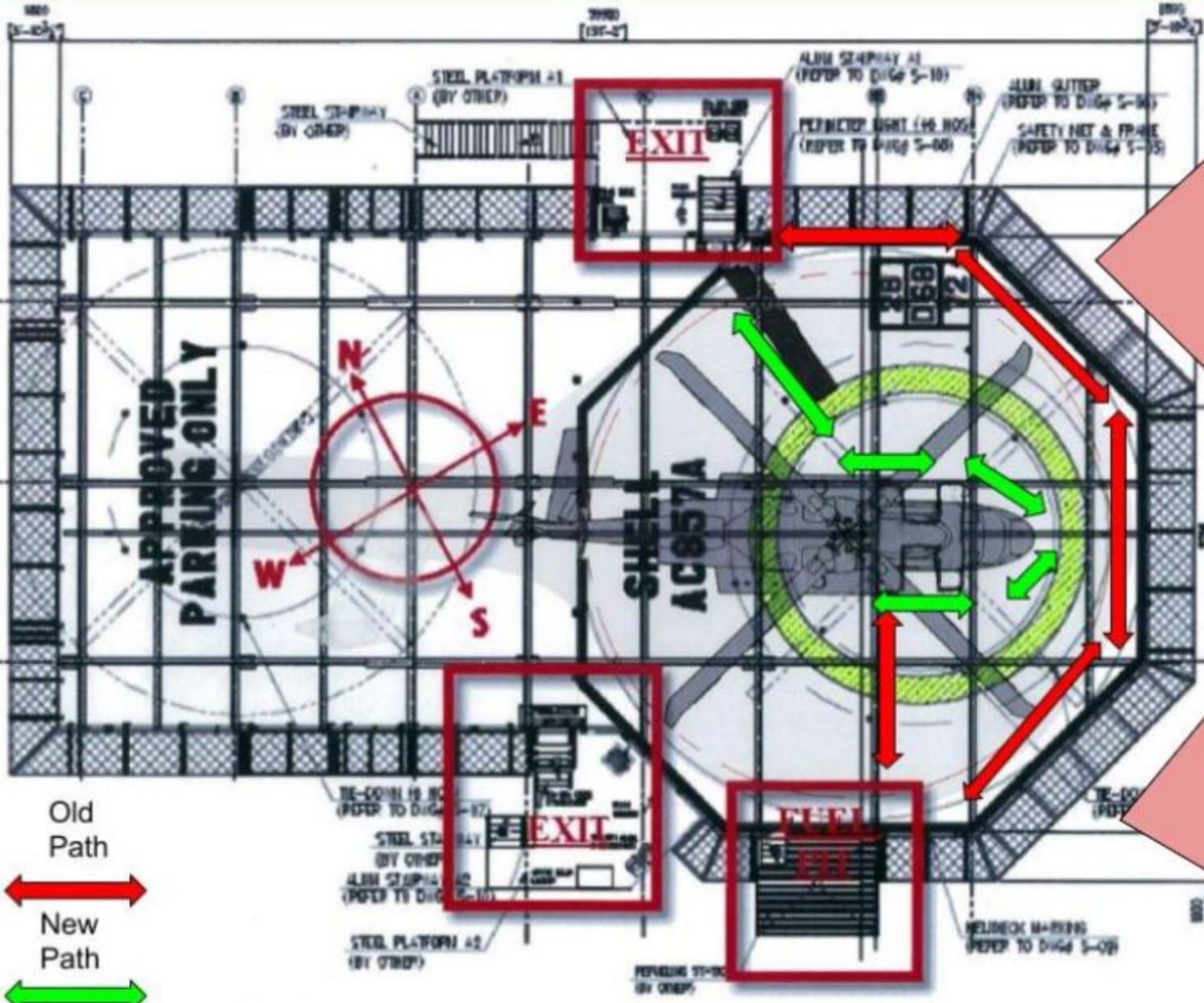
GENERAL LAYOUT
